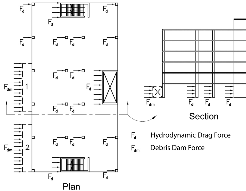
Figure 6-13 Debris dam and drag forces applied to an example building.
