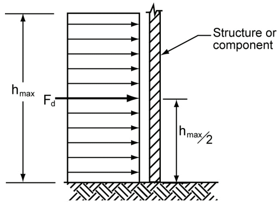
Figure 6-6 Hydrodynamic force distribution and location of resultant.
