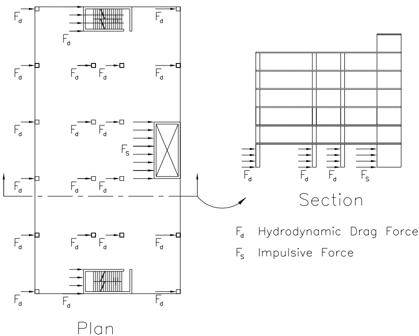
Figure 6-12 Impulsive and drag forces applied to an example building.
