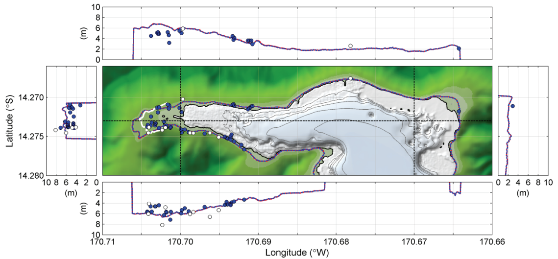
Figure 6-3 Comparison between numerical modeling (blue line) and field measurement of run-up (white dots) and flow elevations (blue dots) at Pago Pago Harbor, American Samoa (Yamazaki et al, 2011).
