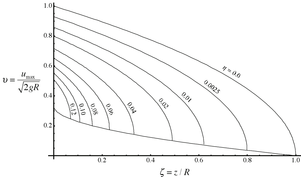
Figure 6-9 Maximum flow velocity of depth, d , at the ground elevation, z , and maximum runup elevation, R . The bottom curve represents the lower limit of maximum flow velocity.
