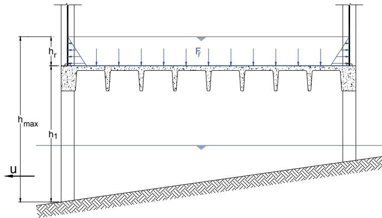
Figure 6-11 Gravity loads exerted on an elevated floor with water retained by exterior walls during rapid drawdown.
