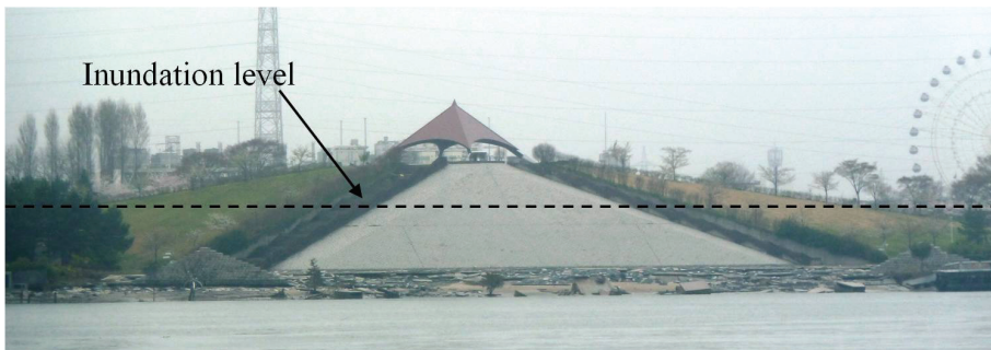
Figure 2-25 Potential evacuation earth mound at West end of Sendai Port (photo courtesy of I. Robertson, ASCE, 2012).
