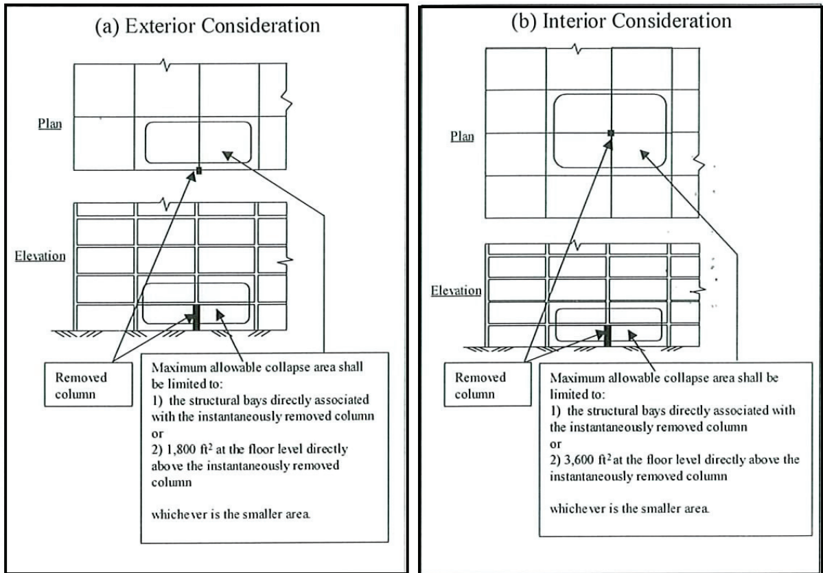
Figure 6-16 Missing column strategy.
