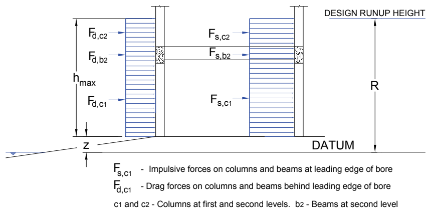
Figure 6-7 Hydrodynamic impulsive and drag forces on components of a building subjected to inundation by a tsunami bore.
