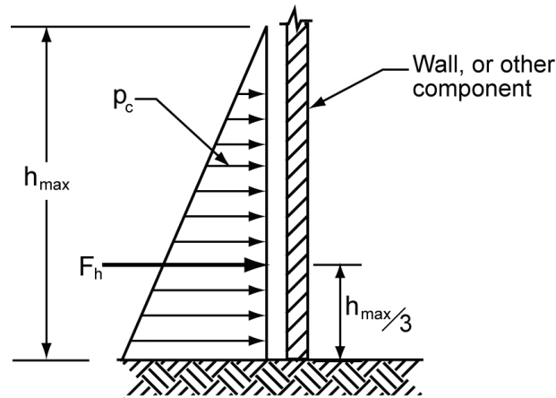
Figure 6-4 Hydrostatic force distribution and location of resultant.
