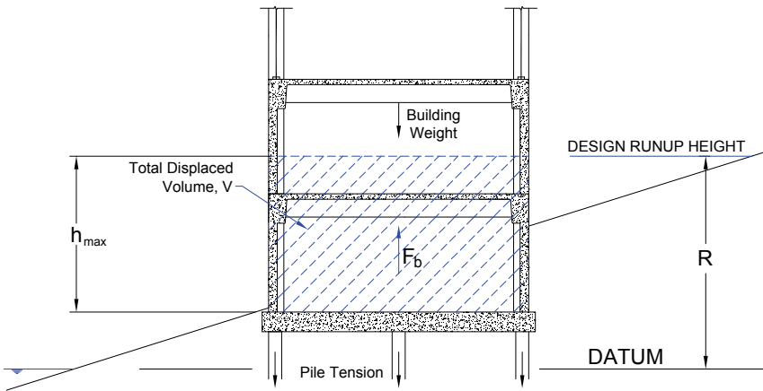
Figure 6-5 Buoyant forces on an overall building with watertight lower levels.
