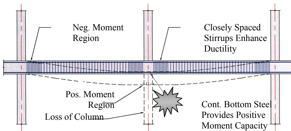
Figure 6-15 Detailing of reinforcing steel for potential loss of a supporting column.
