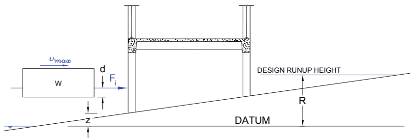
Figure 6-8 Waterborne debris impact force.
