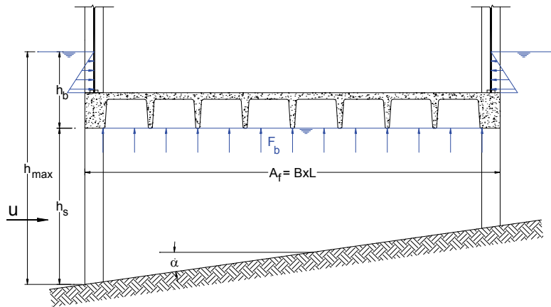
Figure 6-10 A definition sketch for upward buoyant force exerted on an elevated floor.
