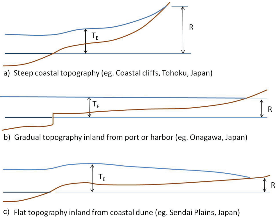
Figure 6-2 Three types of coastal inundation where the tsunami elevation ( T_E ) at a site of interest could be less than, equal to, or greater than the ultimate inland runup elevation ( R )
